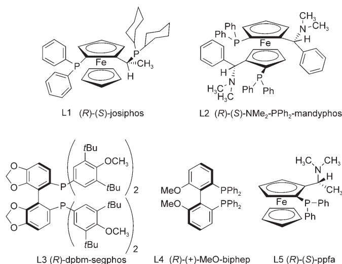
Scheme 1. Structures of ligands.
